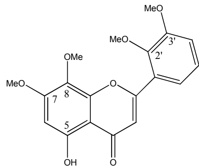
5-hydroxy-7,8,2',3'-tetramethoxyflavone
