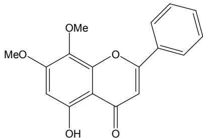
5-hydroxy-7,8-dimethoxyflavone
