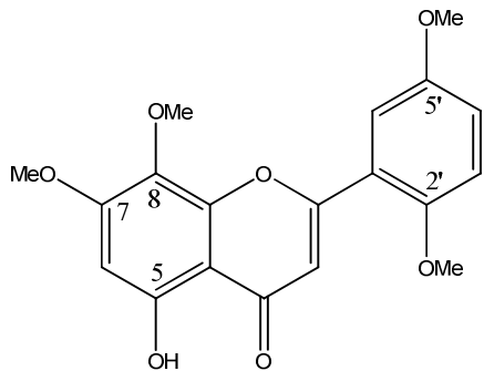
5-hydroxy-7,8,2',5'-tetramethoxyflavone
