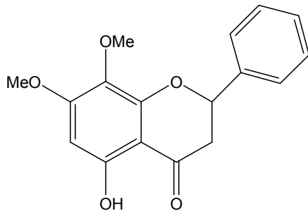
5-hydroxy-7,8-dimethoxyflavanone
