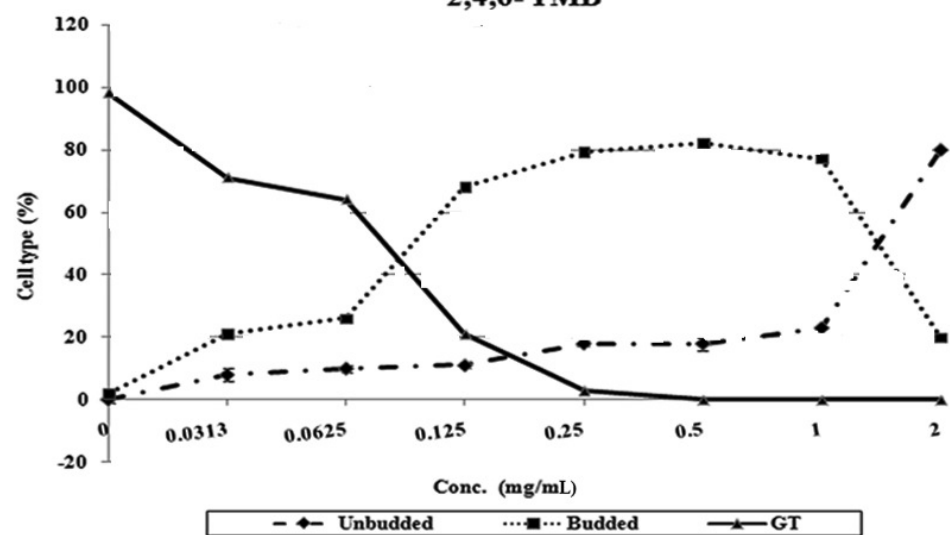
2,4,6-TMB
