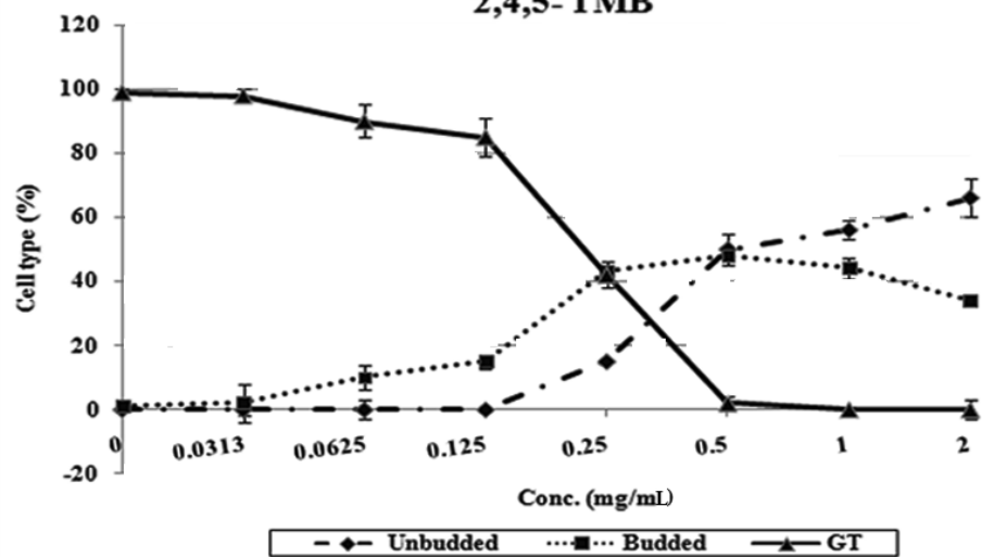
2,4,5-TMB
