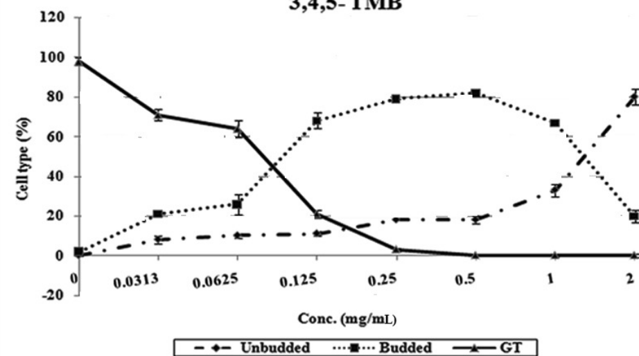
3,4,5-TMB
