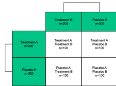
C: factorial
