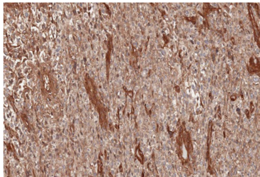
PDGFR-β
