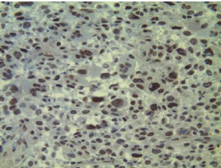
p-mTOR
