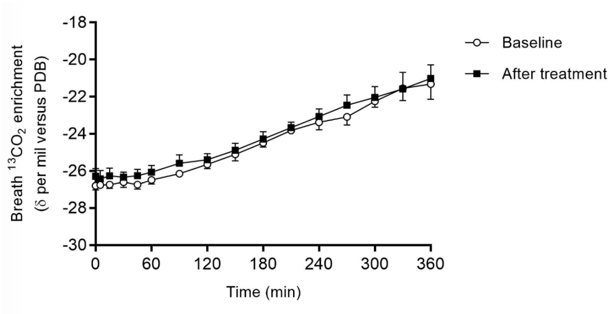
Supplementary Figure S1. Expired breath 13 CO 2 enrichments. Expired breath 13 CO 2 enrichments of the four galactosemia patients, before and after arginine aspartate supplementation. Results are expressed as mean ± SEM.
