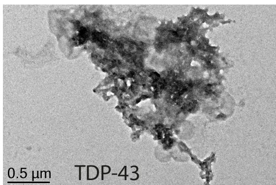
Additional File 12. Morphology of protein aggregates using TEM. Aggregation of purified TDP-43, Htt ex1 -46Q, \alpha -synuclein, \alpha -lactalbumin showing amorphous and fibrillar aggregates. Representative TEM image of endpoint aggregates negatively stained with uranyl acetate, scale bars are as indicated.
