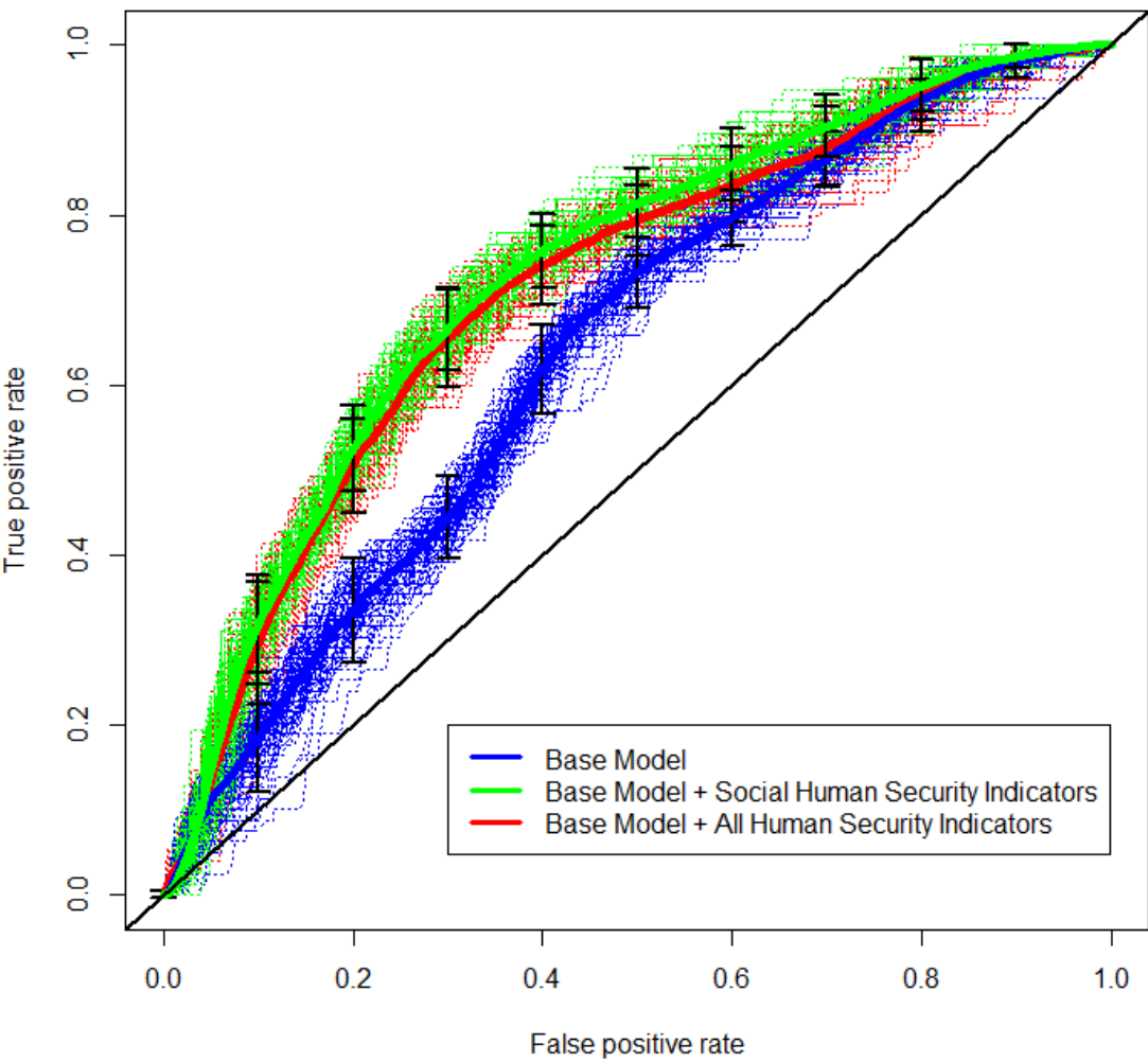
Sexual Violence ROC Curve (6 month)
