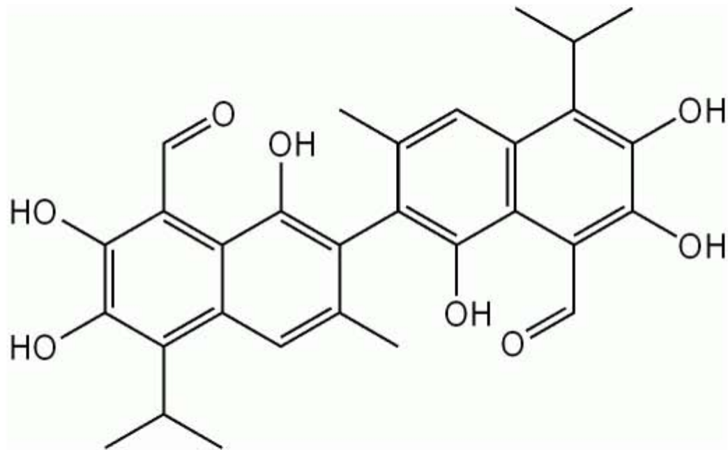
Gossypol
