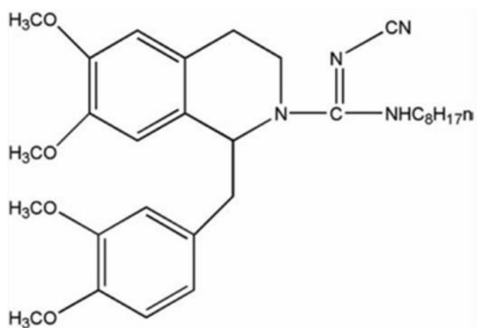
Fig. S1. HZ08 chemical structure.
