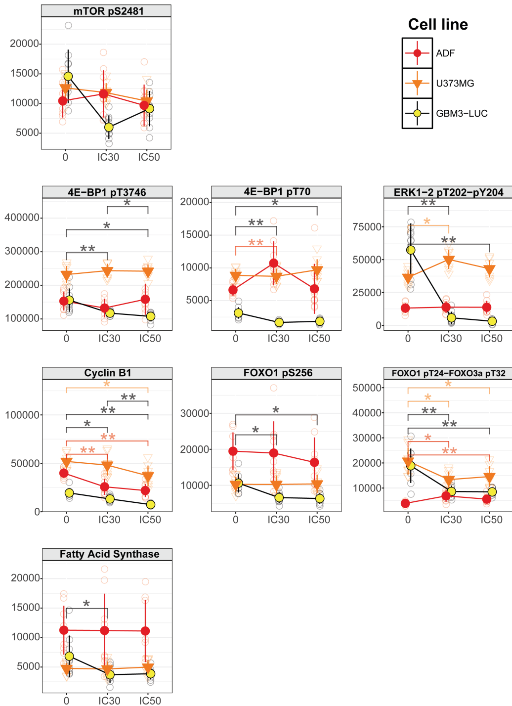
Figure S1. Additional RPPA endpoints. ADF, U373MG and GBM3-Luc cells were incubated with SI113 at the IC30 and IC50 concentrations specific for each cell line and then processed for RPPA analysis. When significant, statistical comparisons (Wilcoxon signed-rank test, FDR-adjusted p values) are reported on each individual plot. Statistical significance coding is described in the Materials and Methods section of the manuscript. RPPA plots refer to results obtained after 2 h (ERK1-2 pT202-pY204) or 8 h (mTOR pS2481, FOXO1 pS256, FOXO1 pT24-FOXO3a pT32 and Fatty Acid Synthase) of exposure to SI113.
