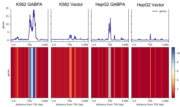
Figure S5. ChIP-seq shows strong GABPA signals on the TGFBR2 promoter in leukemic K562 and liver cancer HepG2 cells. GABPA ChIP-seq results were obtained from GEO dataset (GSM2527661 and GSM2527662) and K562 cells (GSM2825959 and GSM2825960).
