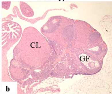
Wild-Type
