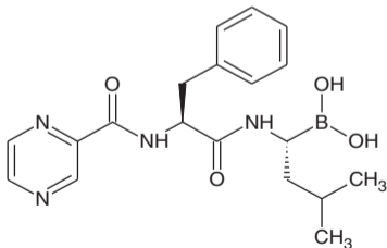
Bortezomib (BORT)
