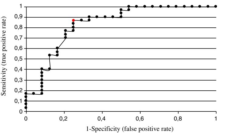
CA125, AUC=0.833
