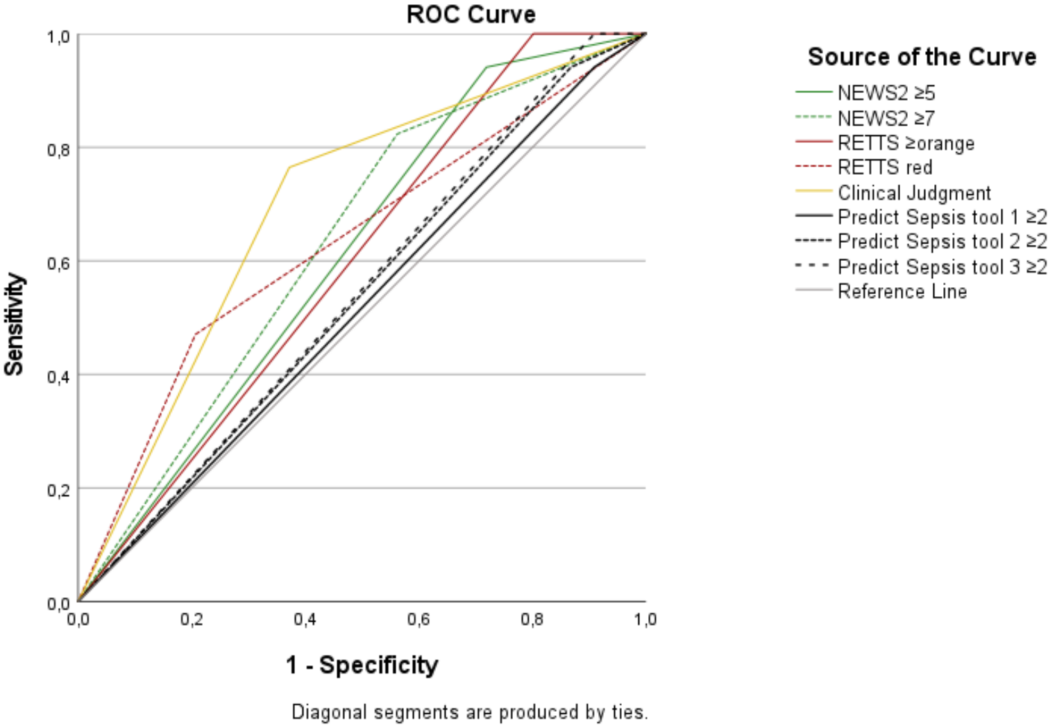
Additional file 12. ROC curves for models with specific cut-offs and septic shock.
