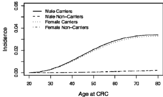
MSH2 mutation
