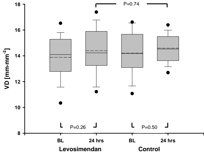
Vessel density
