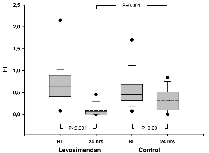
Heterogeneity index
