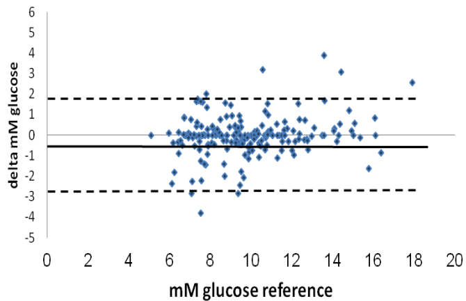
Bland-Altman MD8 glucose
