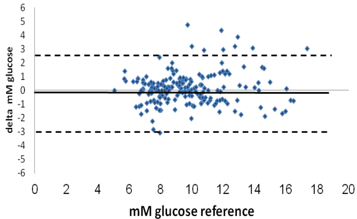
Bland-Altman MD1 glucose
