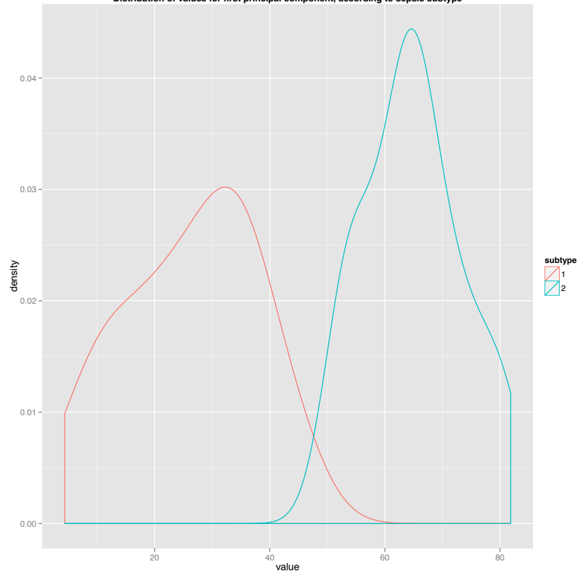
Distribution of values for first principal component, according to sepsis subtype
