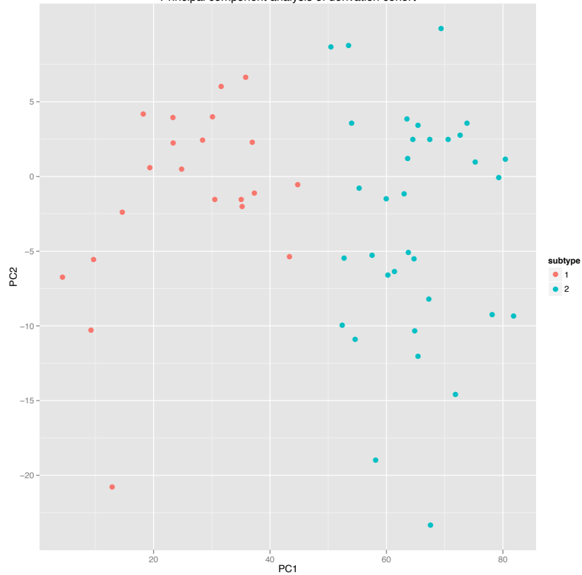
Principal component analysis of derivation cohort
