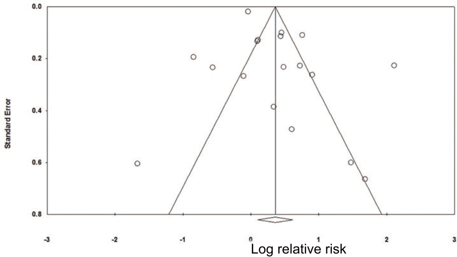
Funnel Plot Standard Error by Log relative risk
