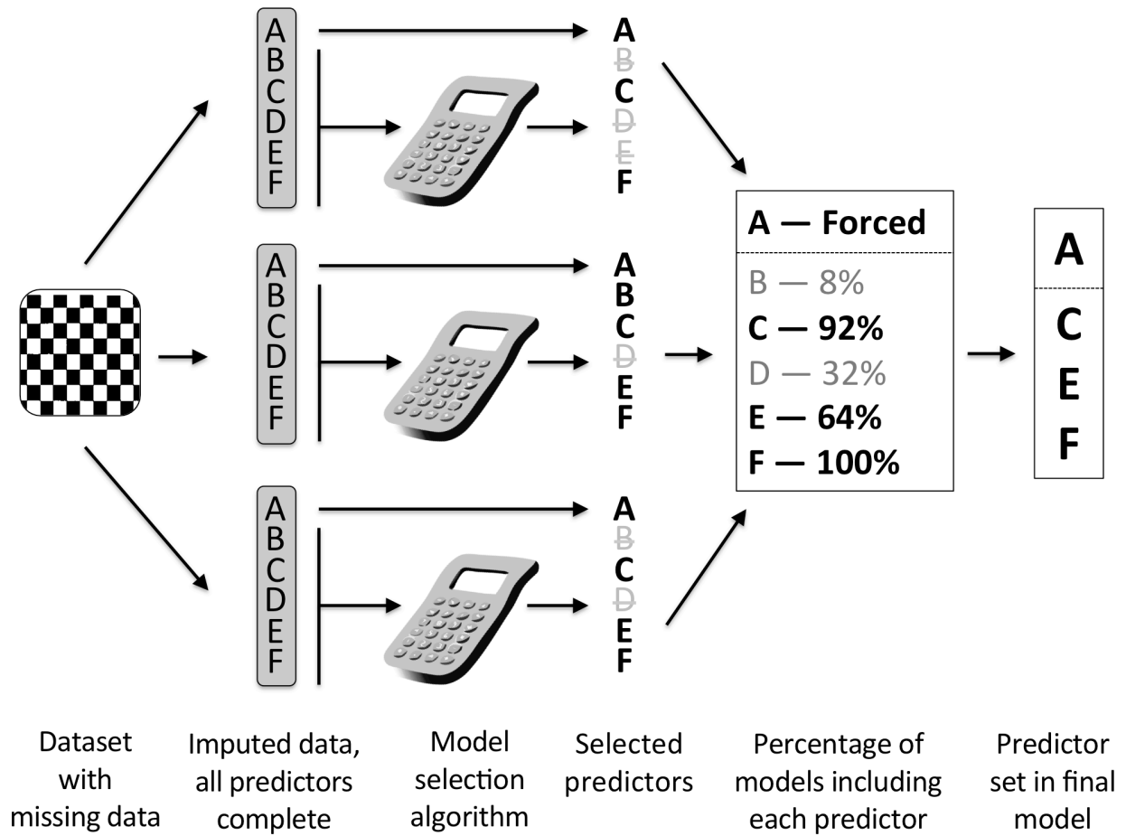
Figure S1. Schematic diagram of “majority rules” model selection algorithm
