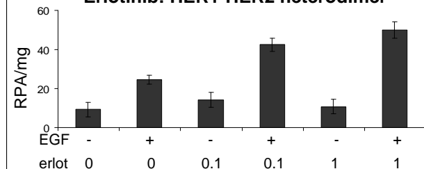
Erlotinib: HER1-HER2 heterodimer
