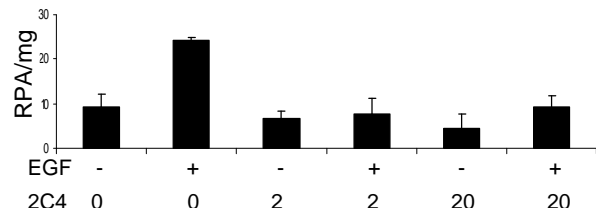
2C4: HER1-HER2 heterodimer
