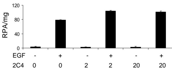
2C4: HER1-HER1 homodimer
