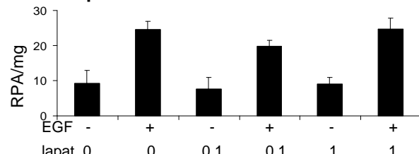
Lapatinib: HER1-HER2 heterodimer
