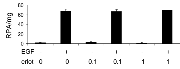
Erlotinib: HER1-HER1 homodimer
