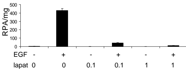
Lapatinib: HER1-HER1 homodimer
