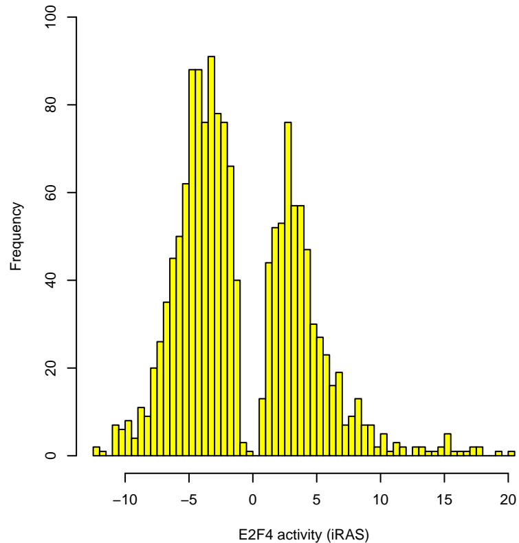
E2F4 activity, ER Positive only n=1485
