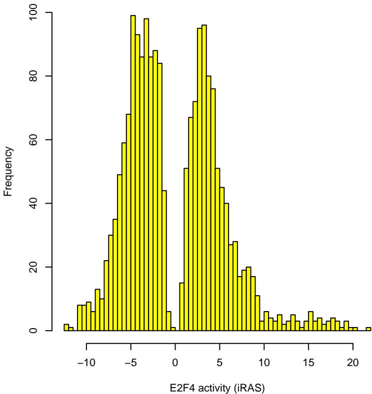
E2F4 activity, all subtypes n=1902
