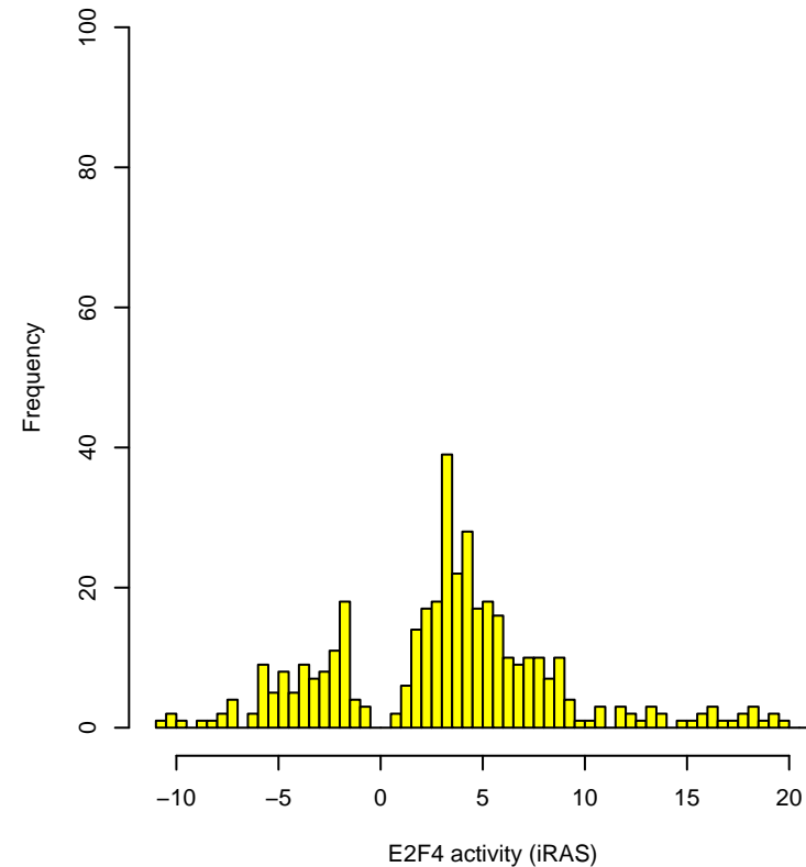
E2F4 activity, ER Negative only n=393
