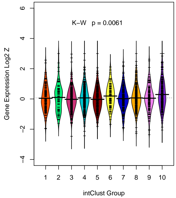
RHCE (ILMN_2408663)
