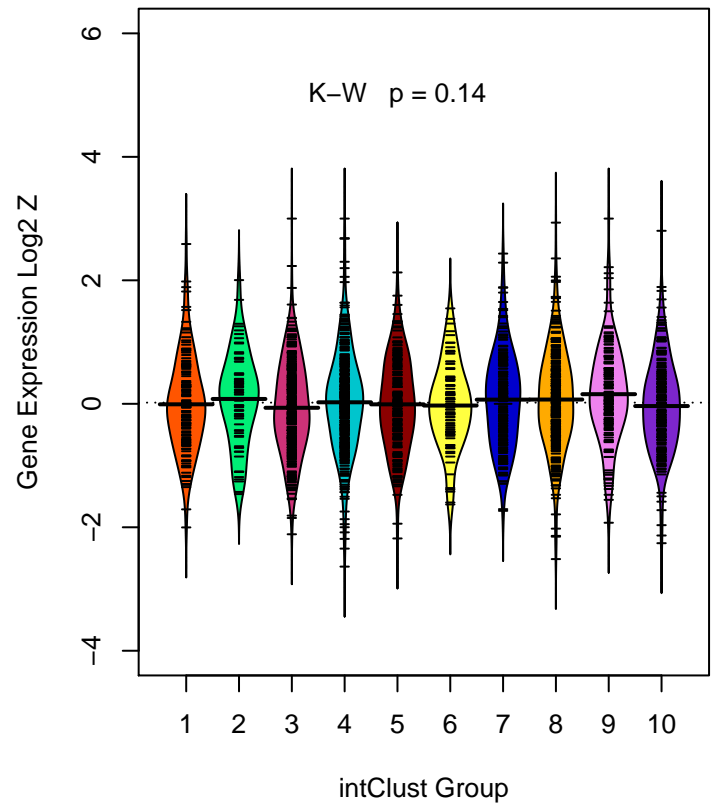
NTN1 (ILMN_1692927)
