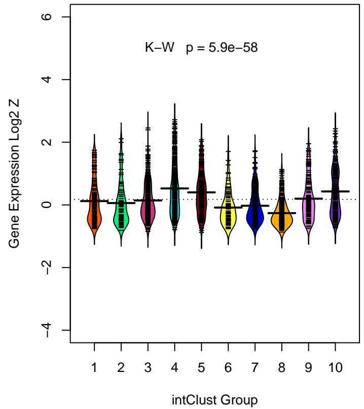
CD79A ( ILMN_1734878 )
