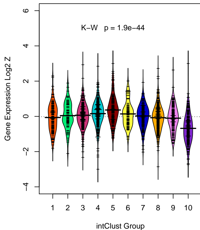
SCARB2 (ILMN_1814726)
