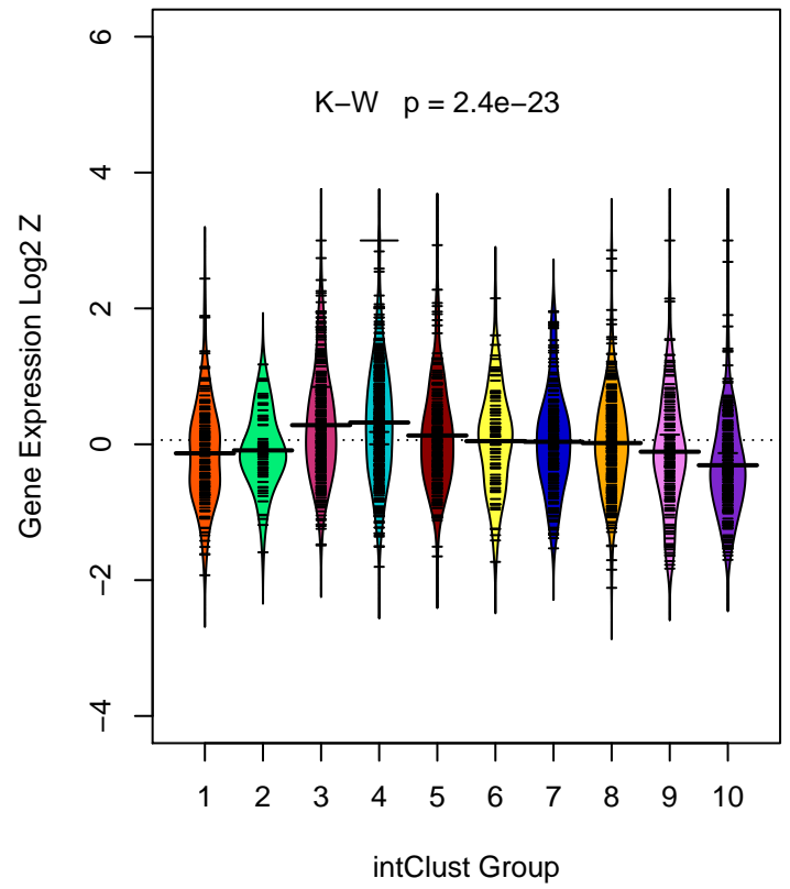
MMP28 (ILMN_1752952)
