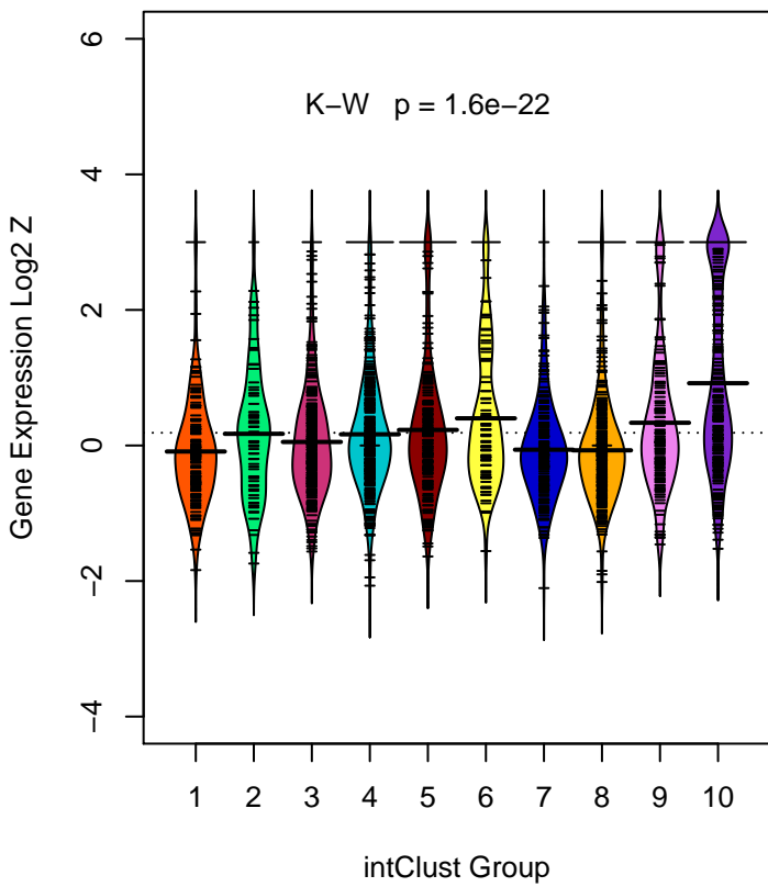
GPR80 (ILMN_1709091)
