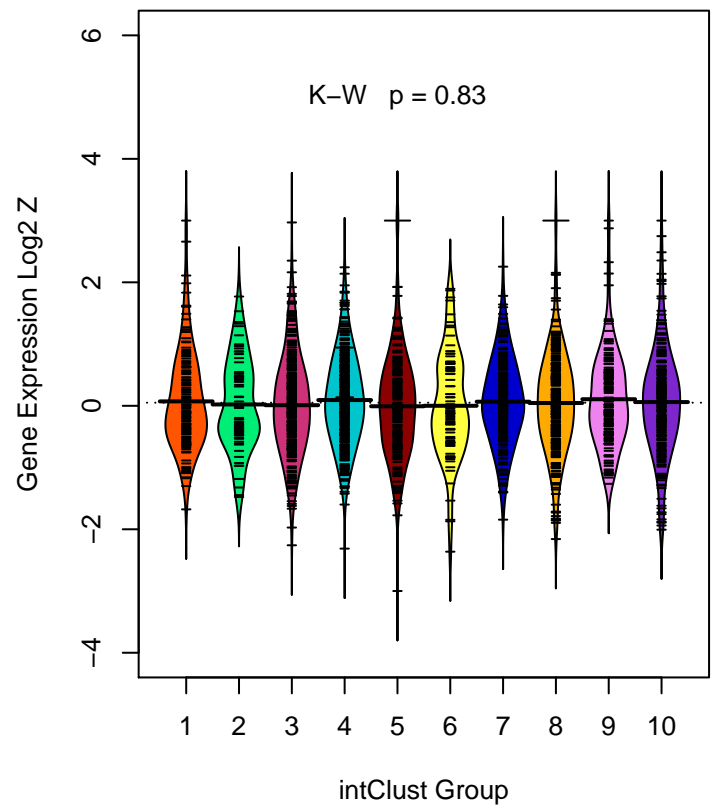
PLUNC (ILMN_1774250)
