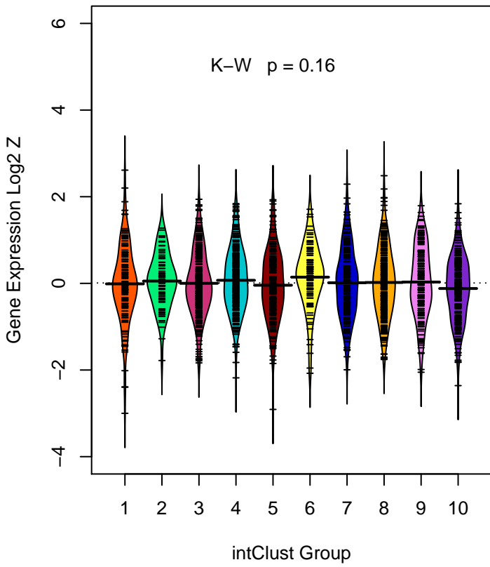
NTN2L (ILMN_1656040)
