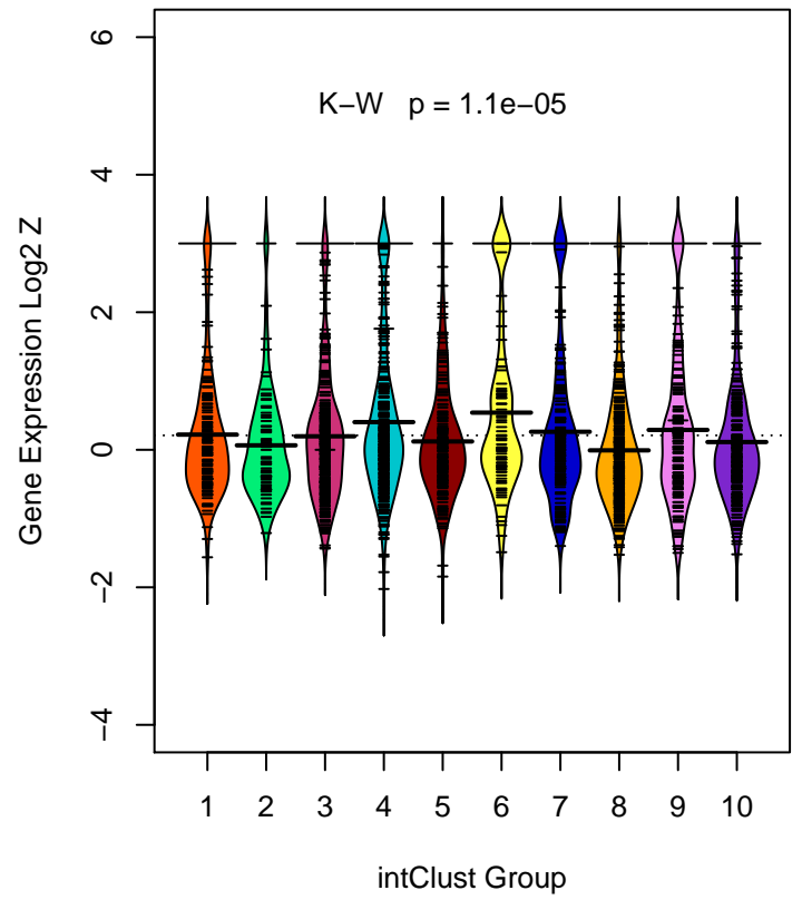
NPTX1 (ILMN_1814221)
