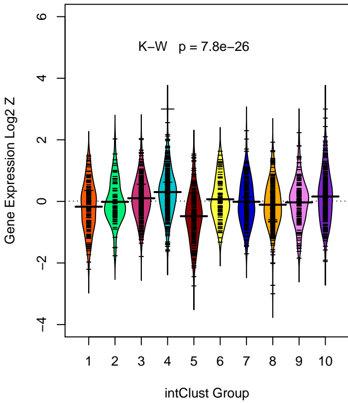
KTELC1 (ILMN_1811104)
