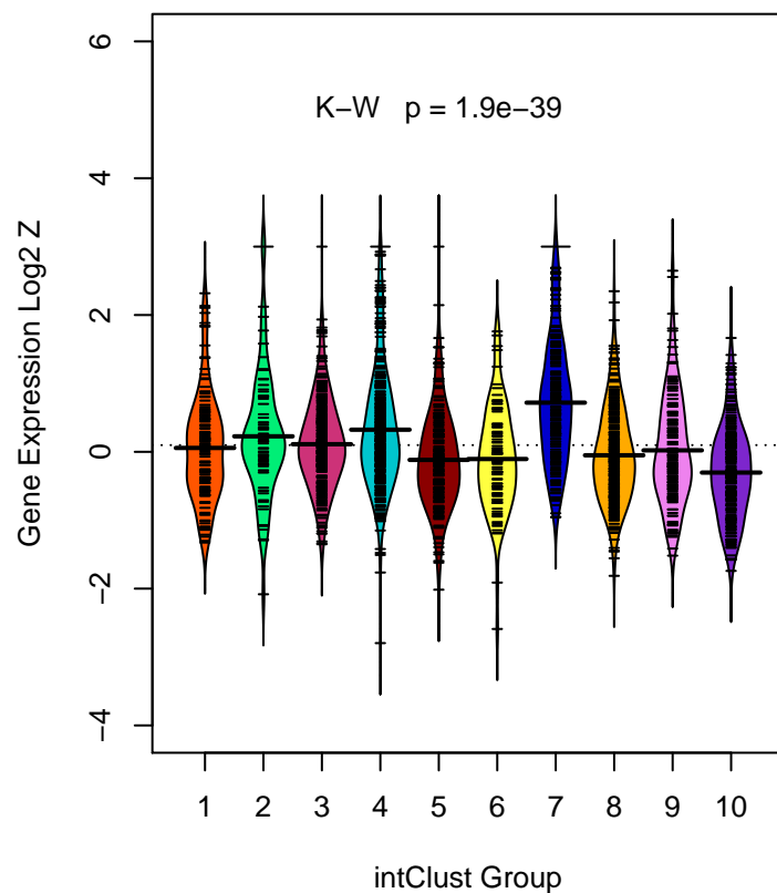
FIT1 (ILMN_1764557)
