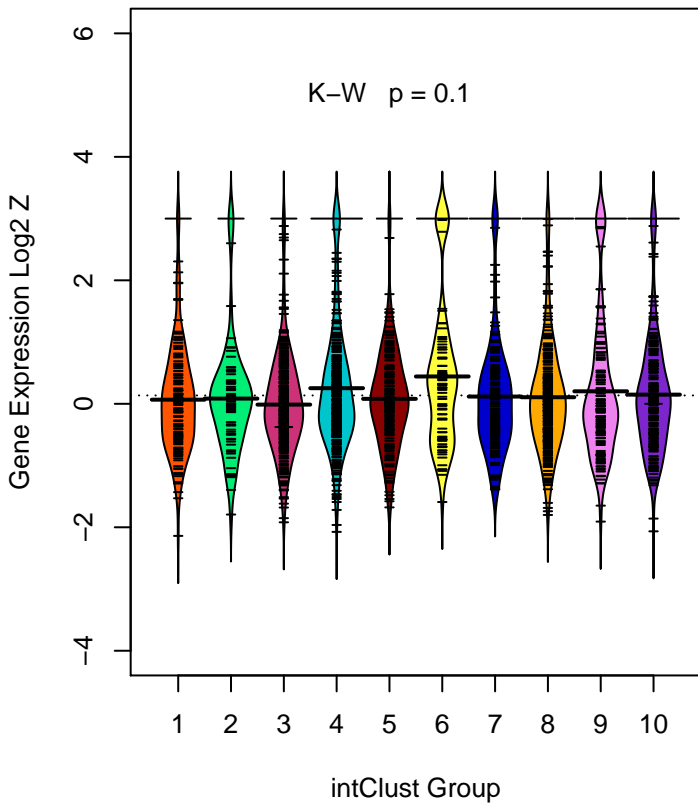
MMP24 (ILMN_1778333)
