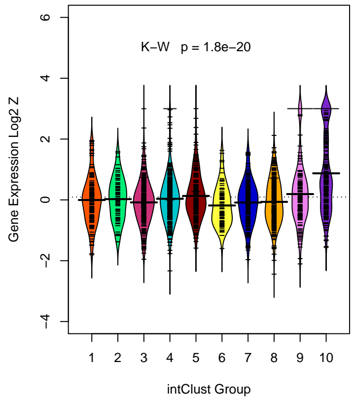
COL9A3 (ILMN_1740155)
