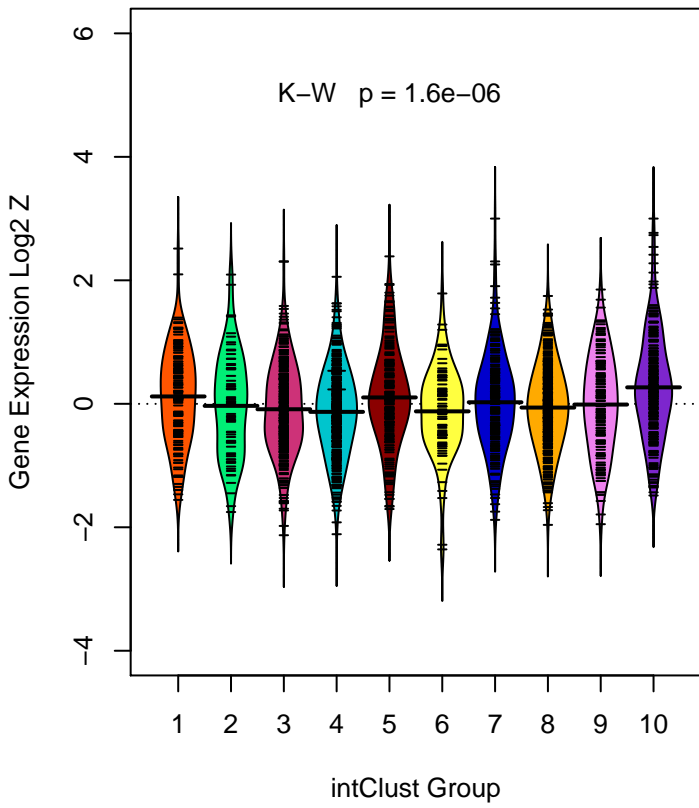
PARD3 (ILMN_1710524)
