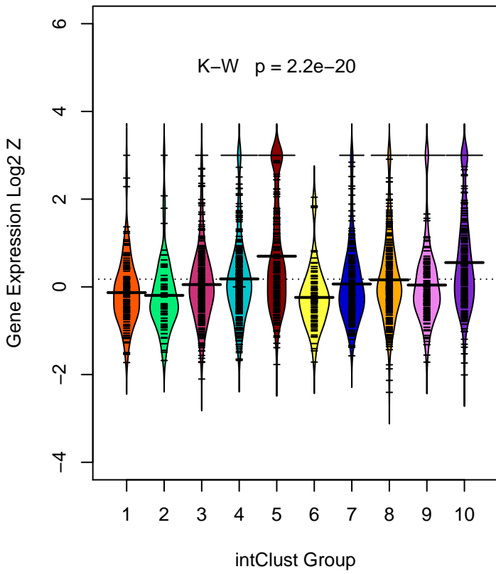
LPAR3 (ILMN_1709719)
