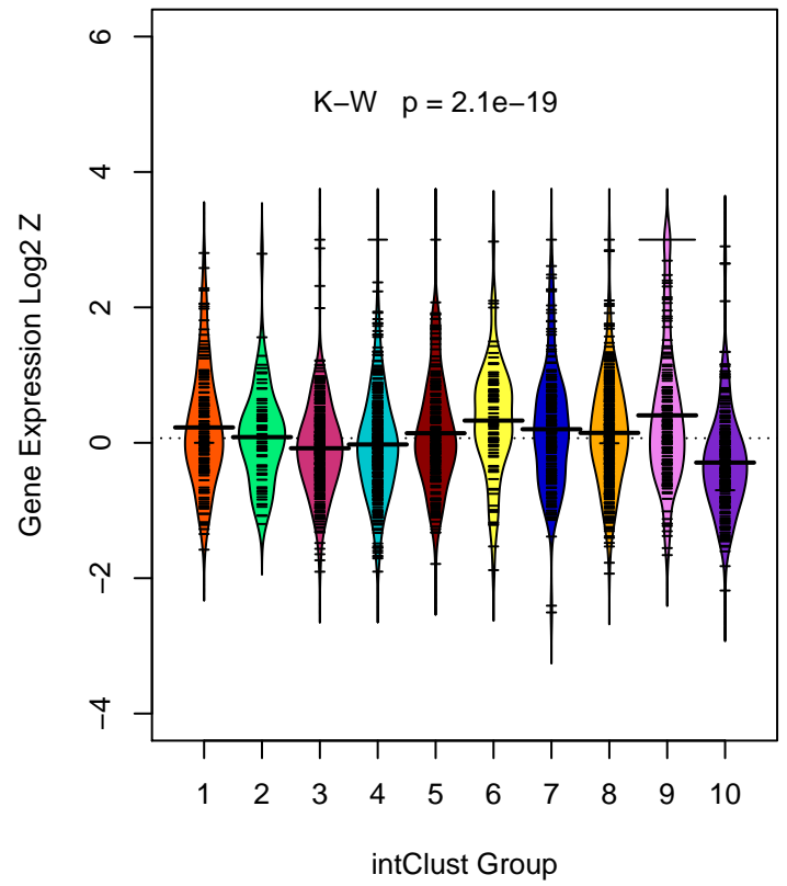
BDKRB2 (ILMN_1684086)
