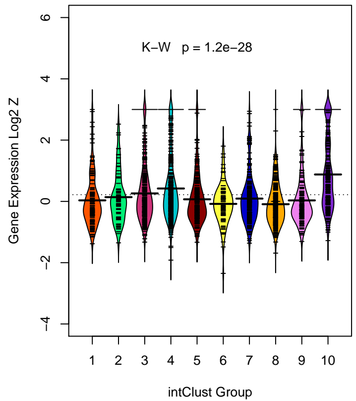
SAA1 ( ILMN_1701017 )
