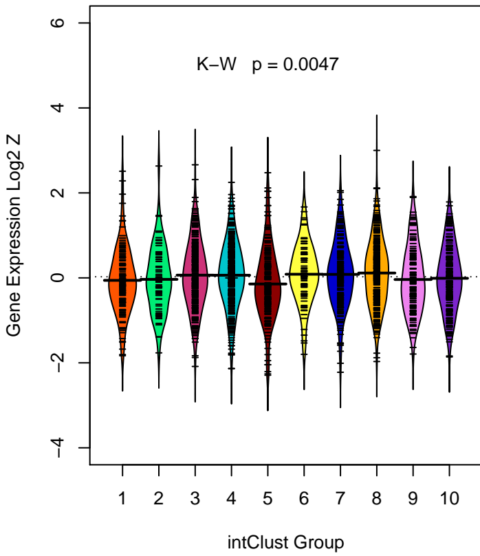
LTBP3 (ILMN_1777121)
