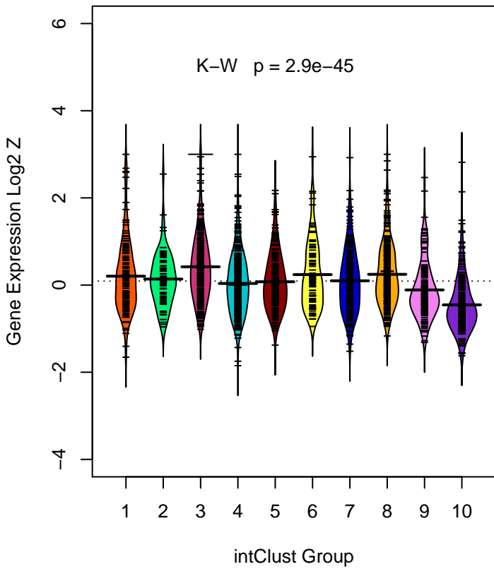
SEMA3C (ILMN_1695475)
