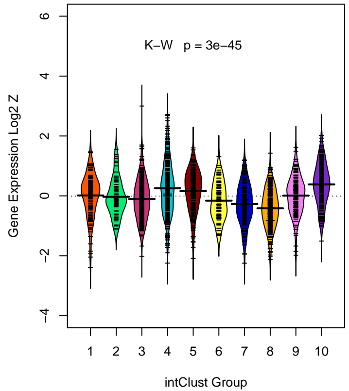
SLC7A7 (ILMN_1810275)
