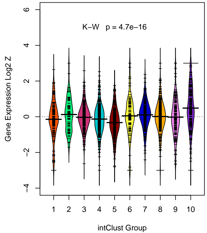
TMEM14C (ILMN_2175131)
