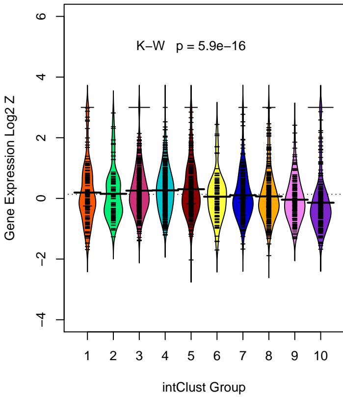
PCDHB13 ( ILMN_1766950 )
