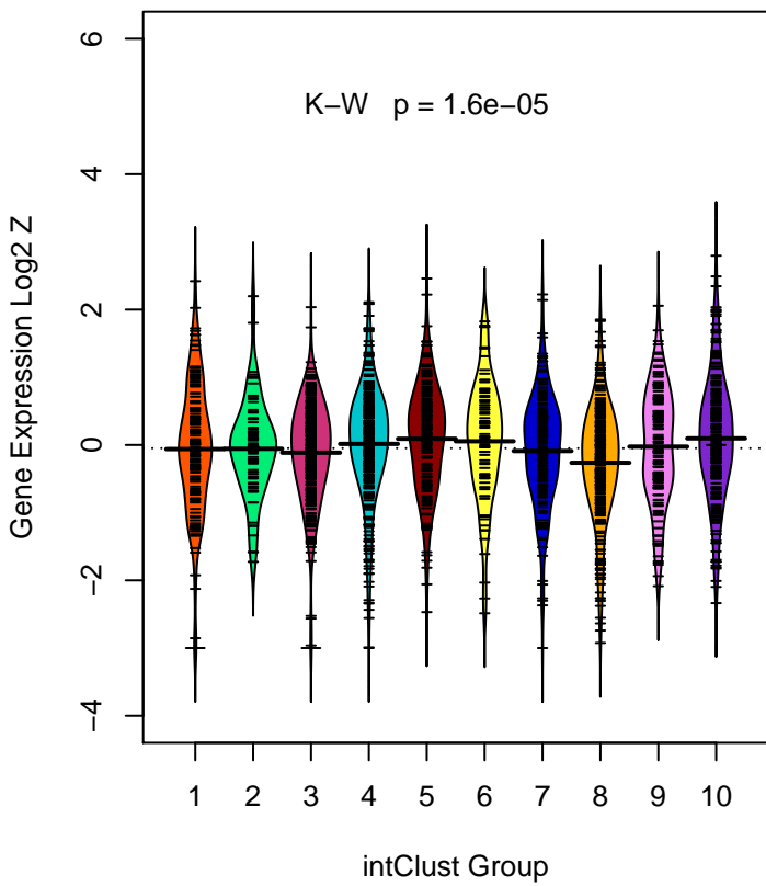
LGALS1 (ILMN_1723978)
