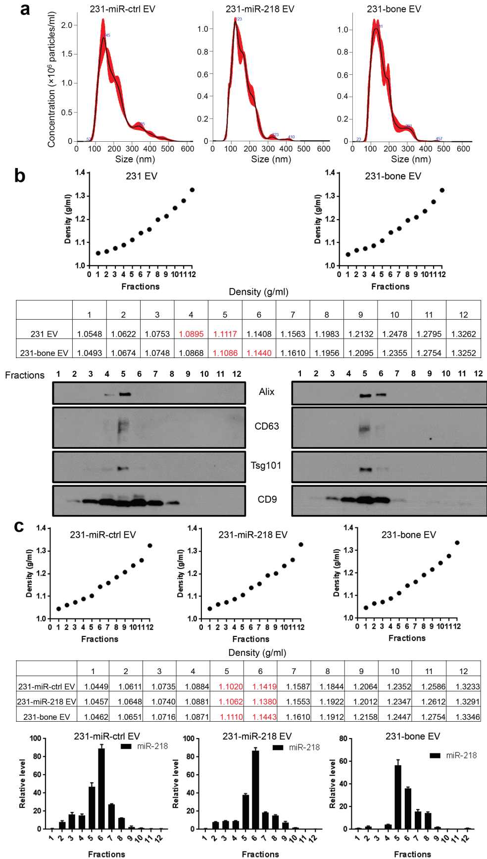
Fig. S1 EV characterization. a EVs pelleted at 110,000 \times g were analyzed by nanoparticle tracking analysis. b Density measurement and Western blot of EV fractions collected from indicated cell lines to detect EV markers. c Density measurement and RT-qPCR of EV fractions collected from indicated cell lines to detect miR-218 levels.
