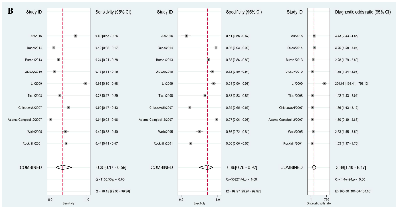
Additional file 15. The pooled sensitivity, specificity and diagnostic odds ratio of the Gail model 1 (A) and Gail model 2 (B).
