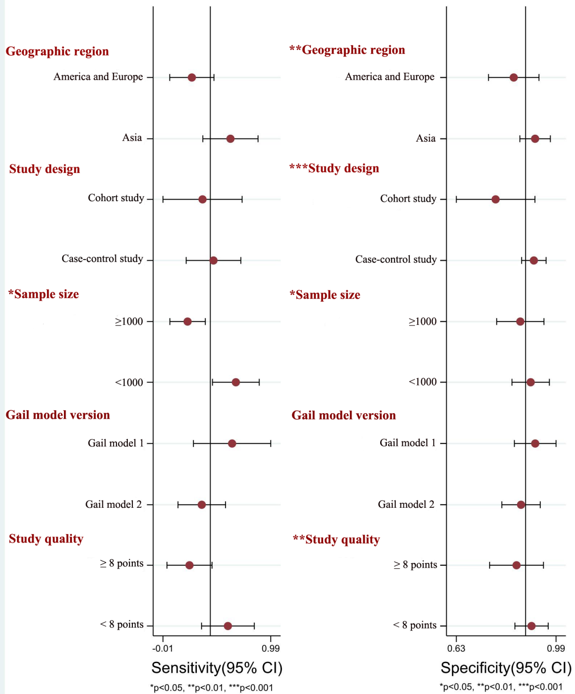
Additional file 17. Subgroup analysis of the diagnostic accuracy of the Gail model.
