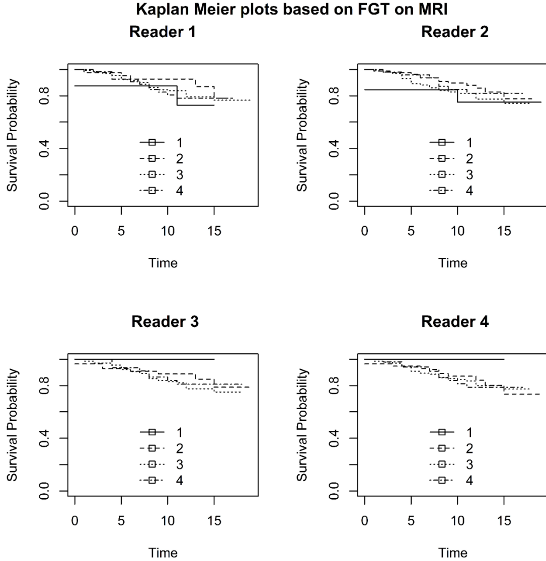
Figure A4: Kaplan–Meier plot of recurrence-free survival using FGT categories on MRI as strata. 1) almost entirely fat; 2) scattered fibroglandular tissue; 3) heterogeneous fibroglandular tissue; 4) extreme fibroglandular tissue.
