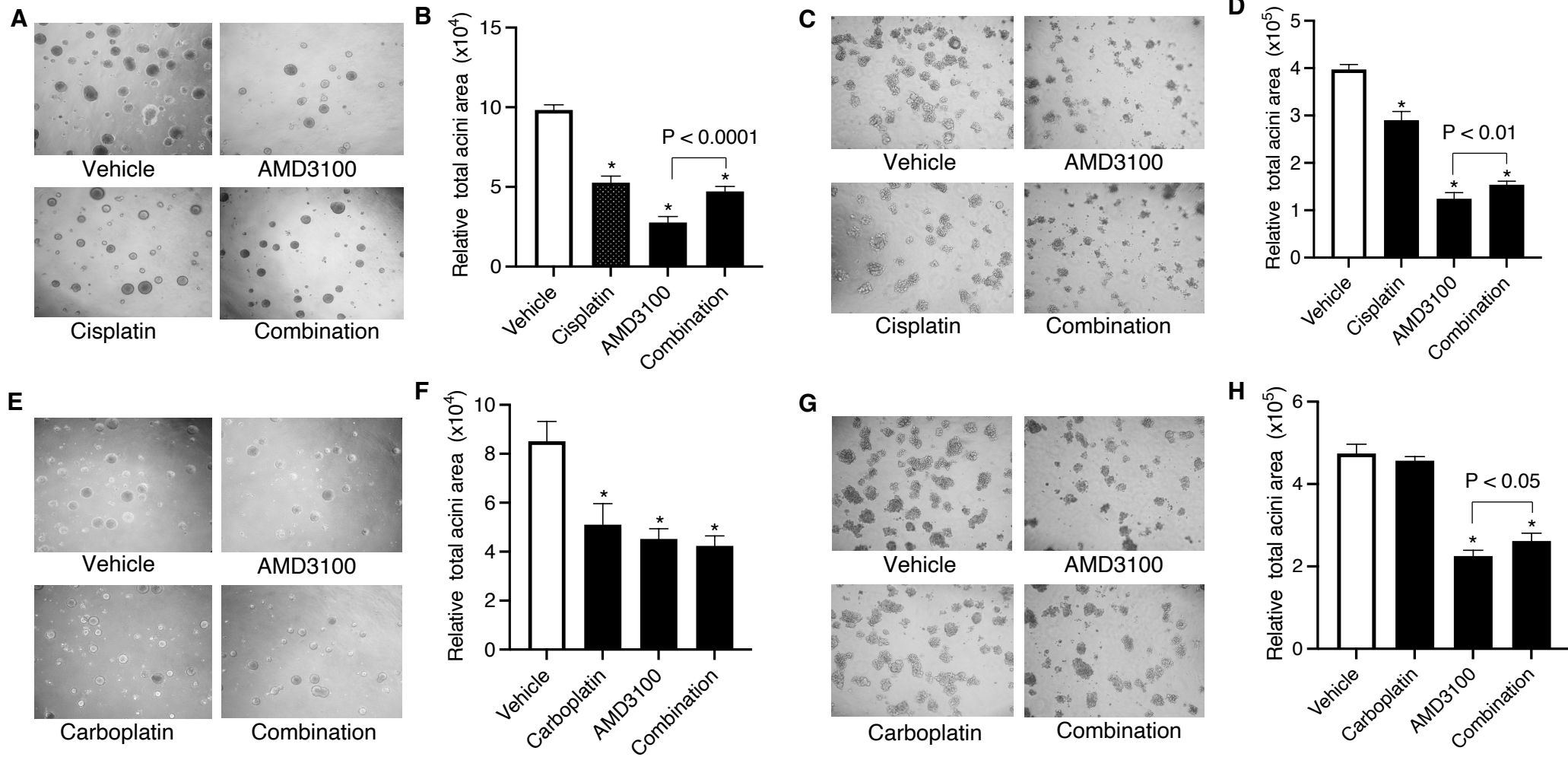
Fig. S7. Effect of combination of AMD3100 and Cisplatin or carboplatin on trastuzumab-resistant breast cancer cell growth. BTRT (A, E) or SKRT cells (C, G) were grown in 3D Matrigel culture and treated with AMD3100 (5 \mu M)/Cisplatin (10 \mu M) (A, C), or AMD3100 (5 \mu M)/Carboplatin (10 \mu M) (E, G). Photographs were taken on day 11. Quantitative analysis of the total acini area was performed using AlphaView SA, and the data were analyzed using one-way ANOVA (B, D, F, H: *, P < 0.0001 vs. Vehicle).
