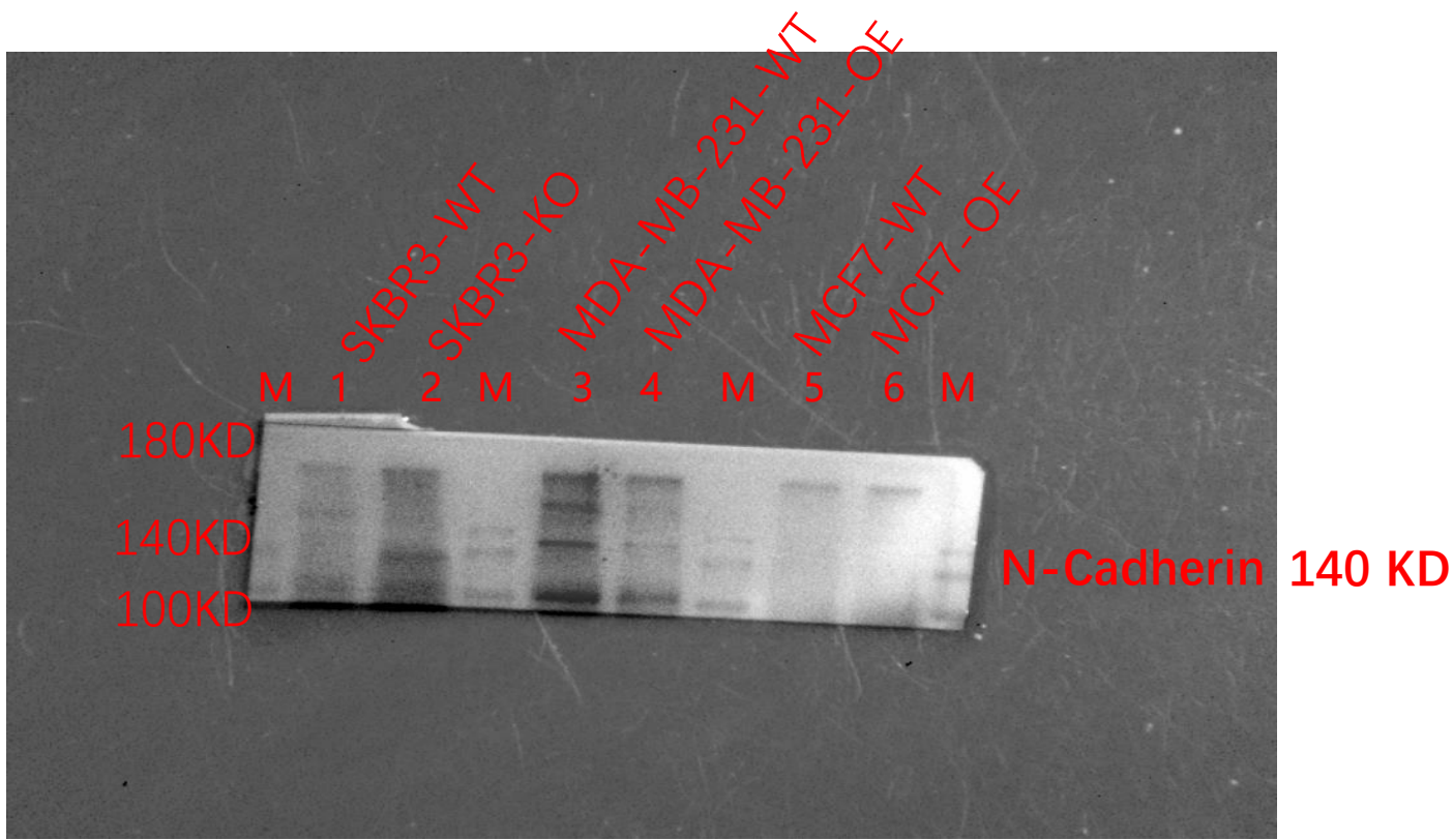
Fig.S3D-N-cadherin
