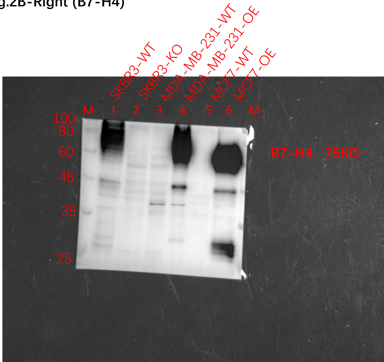
Fig.2B-Right (B7-H4)
