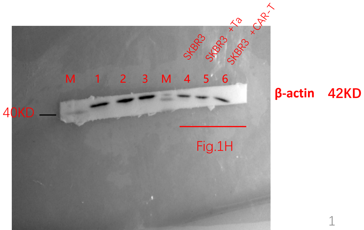
Fig.1H-(actin)
