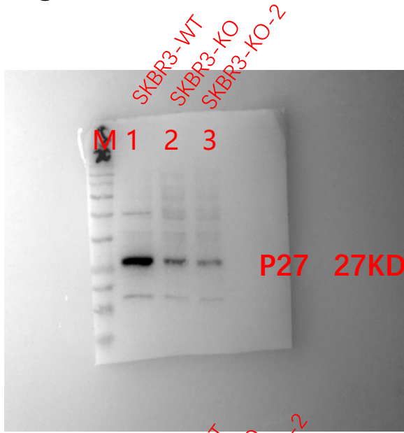
Fig.S2D
