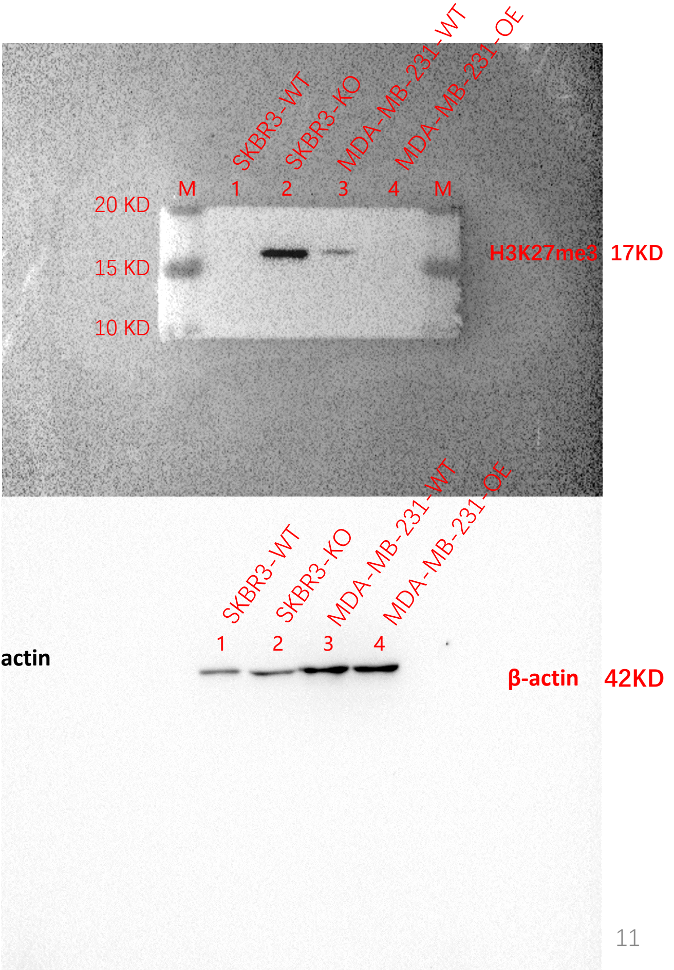
Fig.S4F-H3K27me3
