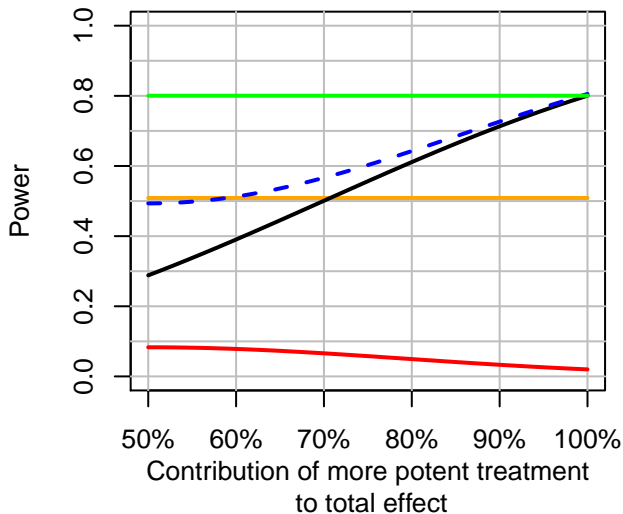
Sample size = 750
