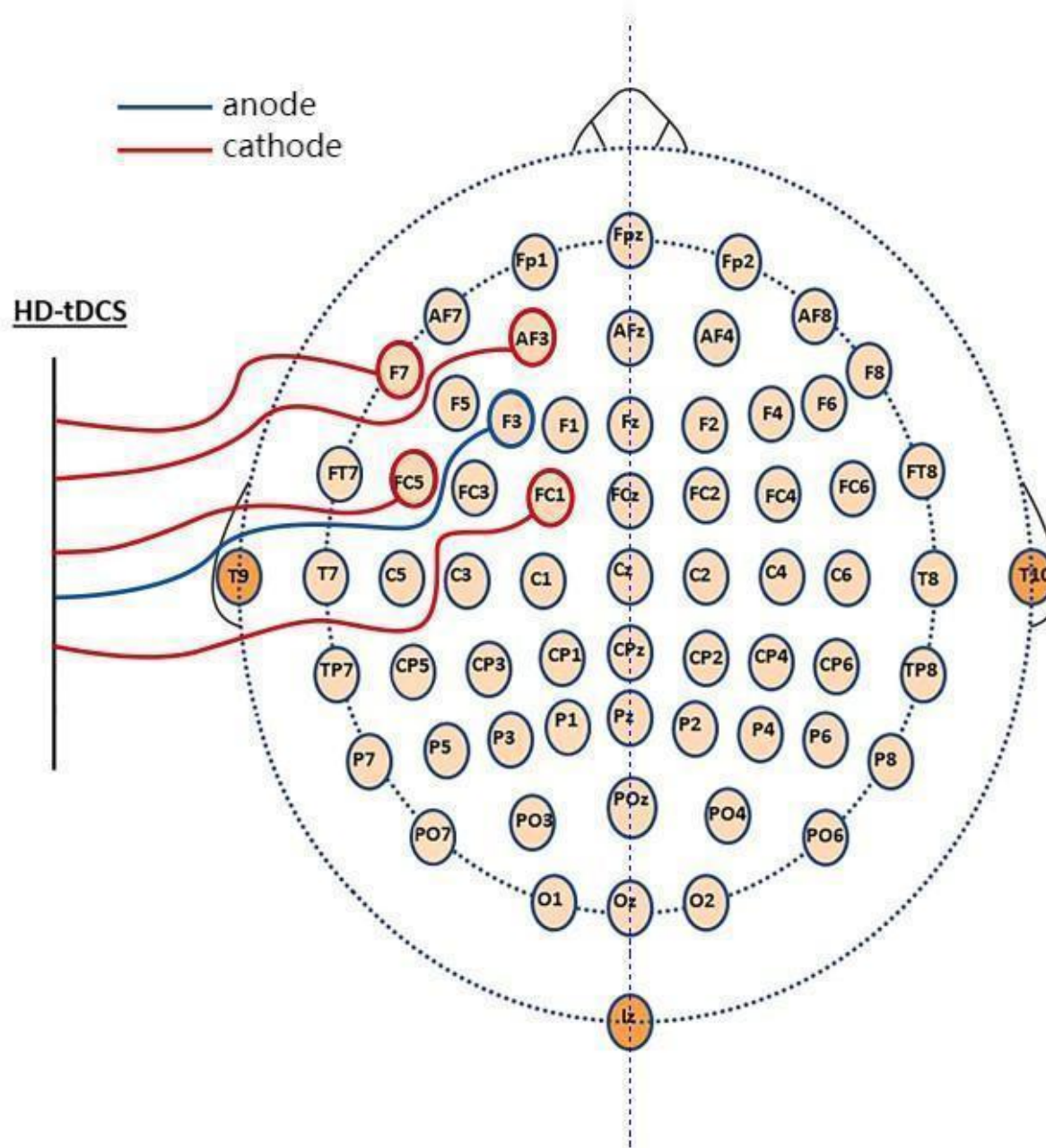
Additional file 1. HD-tDCS setting of electrode annotations
