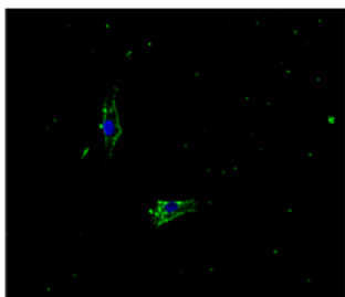
Chicken IgY
