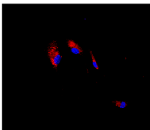
CD45
