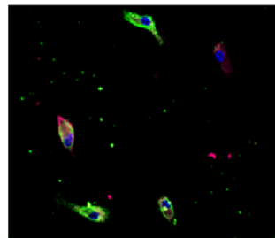
CCR2 & CD45
