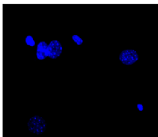
Rabbit IgG
