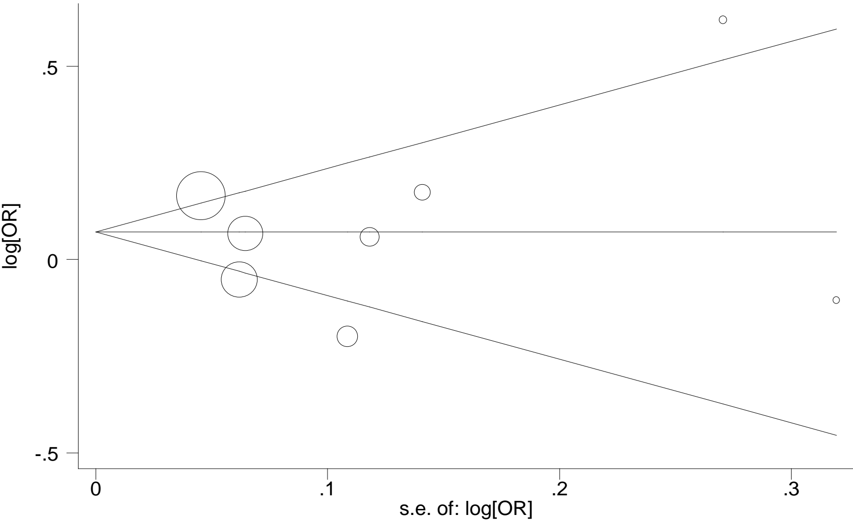
Begg's funnel plot with pseudo 90% confidence limits
