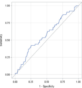
Adiponectin AUC=0.57
