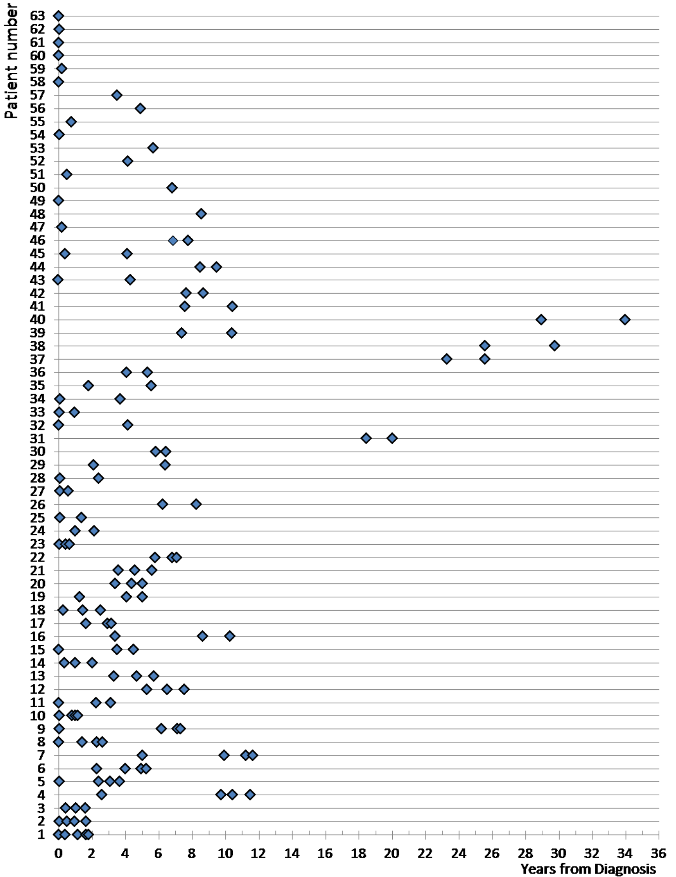
Additional Figure 1.: Unbalanced design of data collection. Samples analyzed with HLM are highlighted by background.
