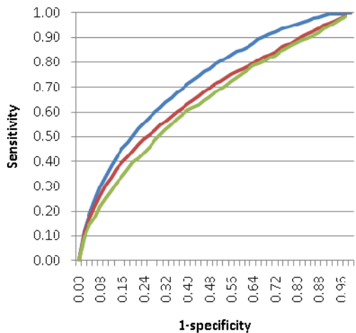
Scen1 (Recessive)
