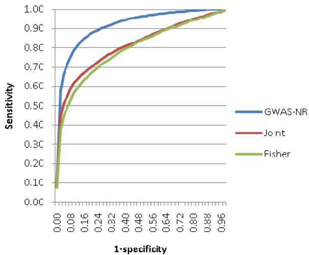
Scen1 (Multiplicative)
