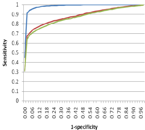
Scen1 (Dominant)
