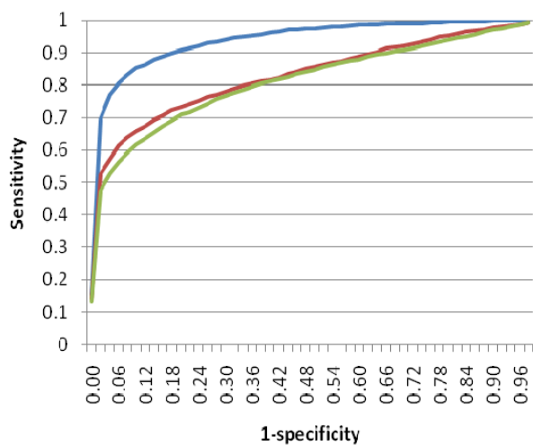
Scen1 (Additive)
