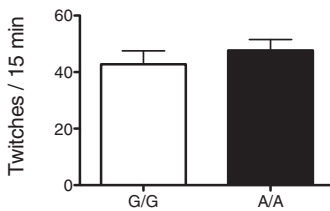
E DOI-Induced Head Twitch Response
