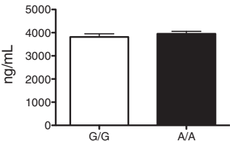
C Synaptosome uptake (20nM 5-HT)
