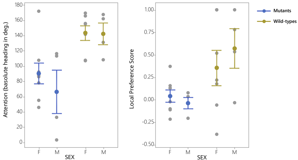
Figure S1: Comparisons of males (M) to females (F) of shank3a mutants and their wild-type siblings in attention towards distress during observation and local preference at the test phase of the behavioural experiment
