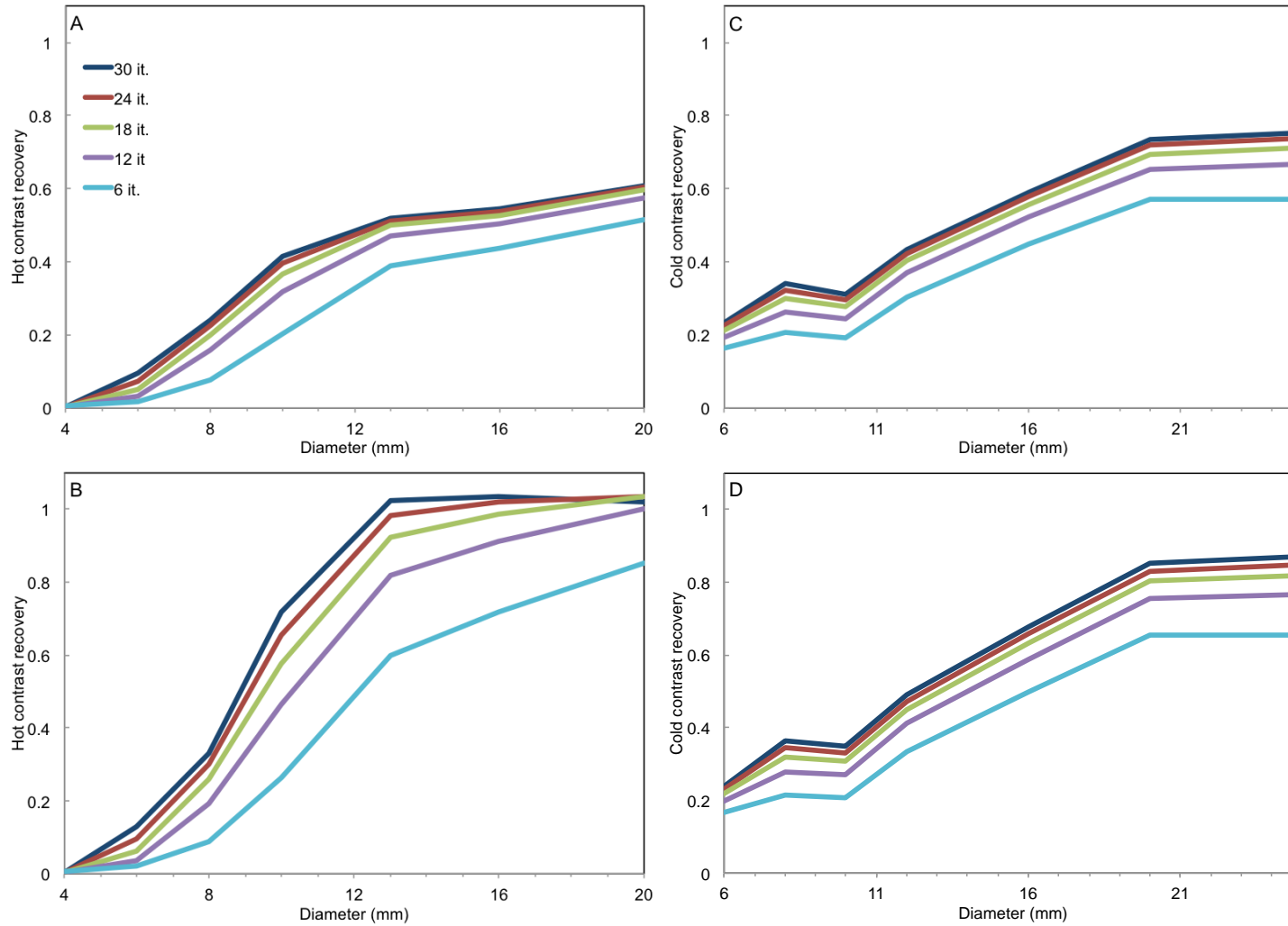
Supplementary Figure 8. Contrast recovery in function of the number of iterations for General Electric Infinia Hawkeye 4. Reconstructions were performed with General Electric Evolution for Bone including attenuation and scatter correction and resolution recovery and eight subsets. (A, B) Hot rods. (C, D) Cold rods. (A, C) Full ROI. (B, D) Half ROI.
