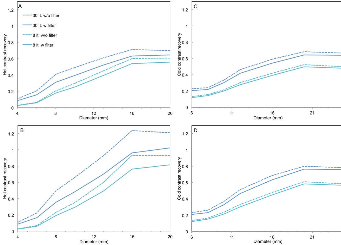
Supplementary Figure 10. Contrast recovery with and without post filter for Siemens Symbia T6. Reconstructions were performed with Siemens Flash3D including attenuation and scatter correction and resolution recovery and eight subsets. (A, B) Hot rods. (C, D) Cold rods. (A, C) Full ROI. (B, D) Half ROI.
