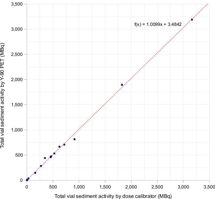
Total vial sediment activity by Y-90 PET vs dose calibrator
