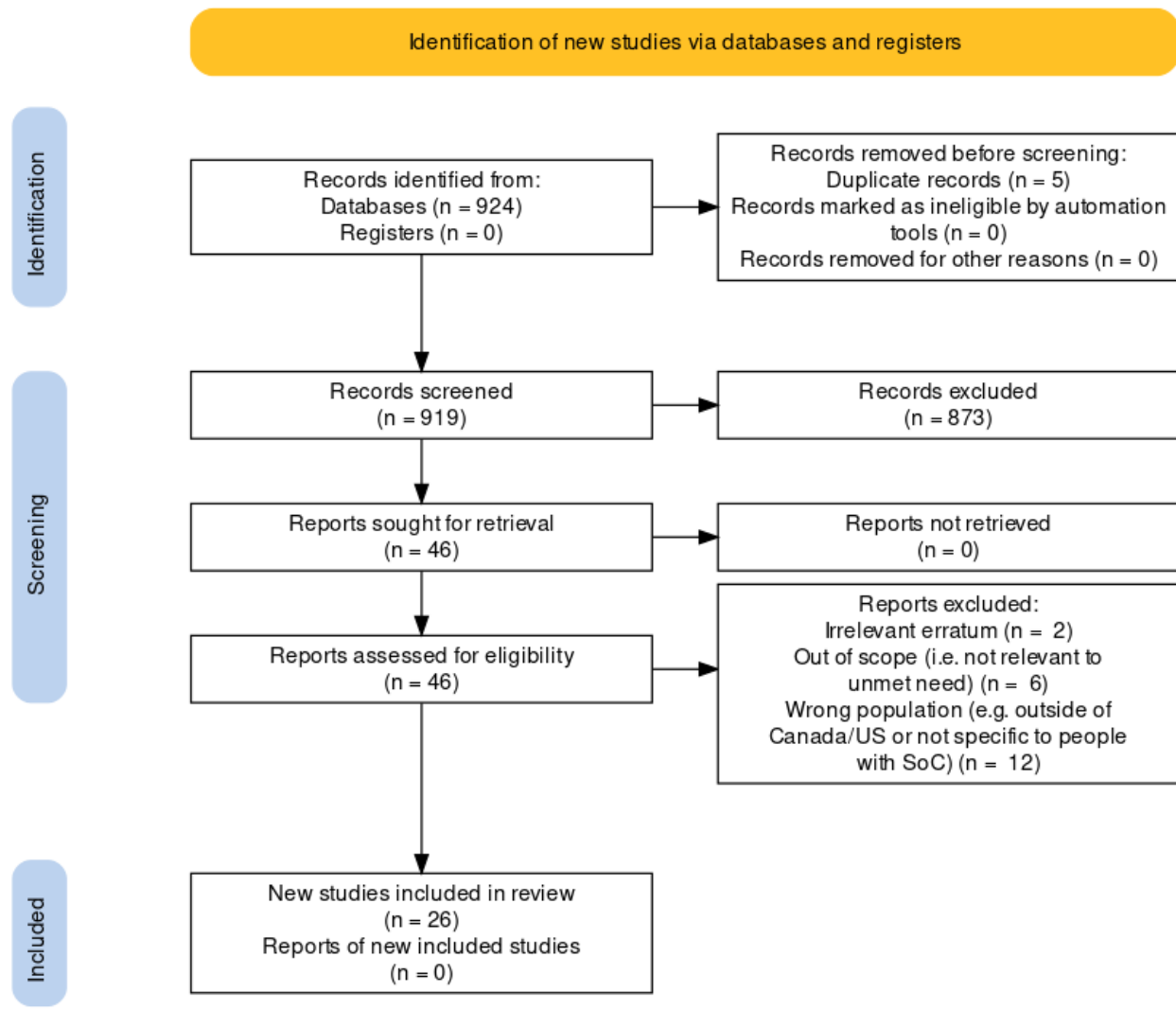
Fig. S1 PRISMA flow diagram
