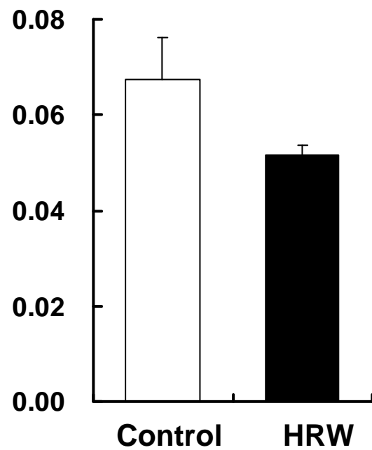
(f) 3-deoxyglucosone
