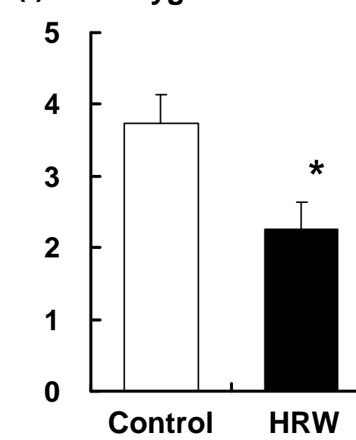
(f) 3-deoxyglucosone
