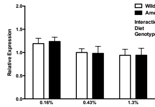
Muscle Gcic
