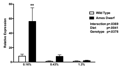
Muscle Mat1a
