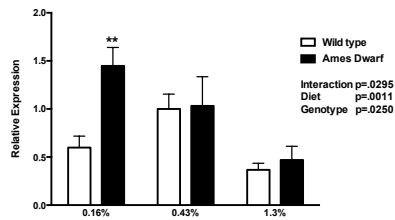
Muscle Bhmt
