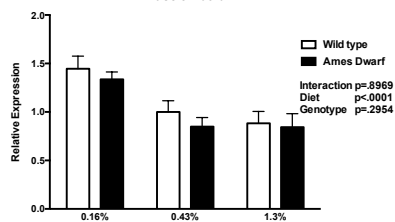
Muscle Mat2a
