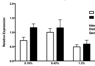
Muscle Ahcy
