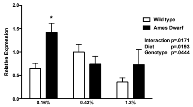
Muscle Mthfr
