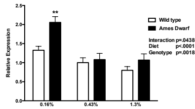
Muscle Mtr
