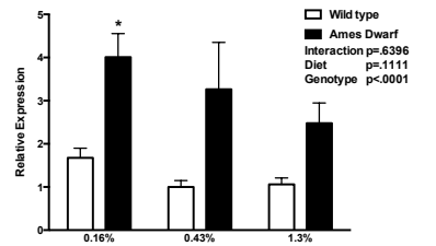
Muscle Cth
