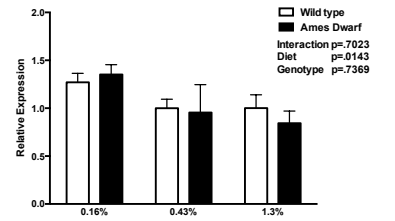
Muscle Gcim
