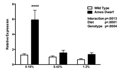
Muscle Cbs
