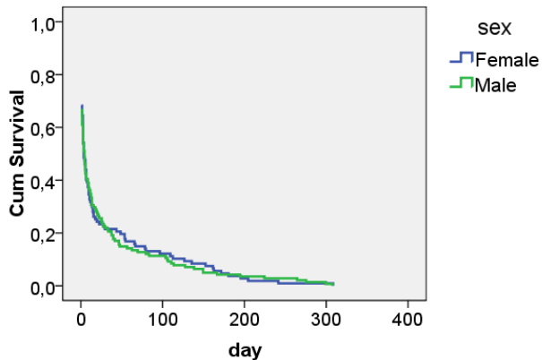
Survival Functions
