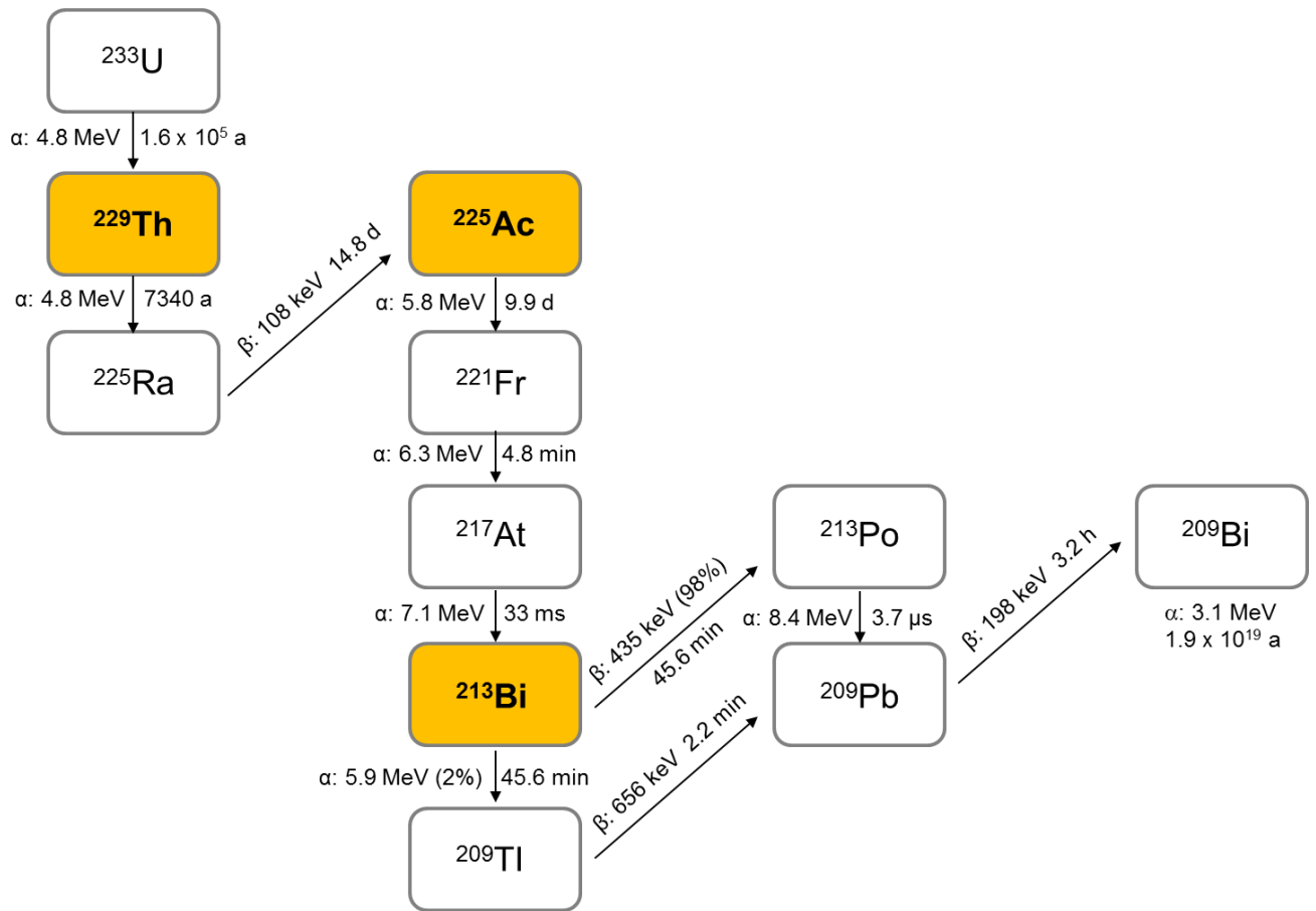
Supplement Figure 2: Decay schema of the ^{229}\text{Th} / ^{225}\text{Ac} / ^{213}\text{Bi} radionuclide generator system
