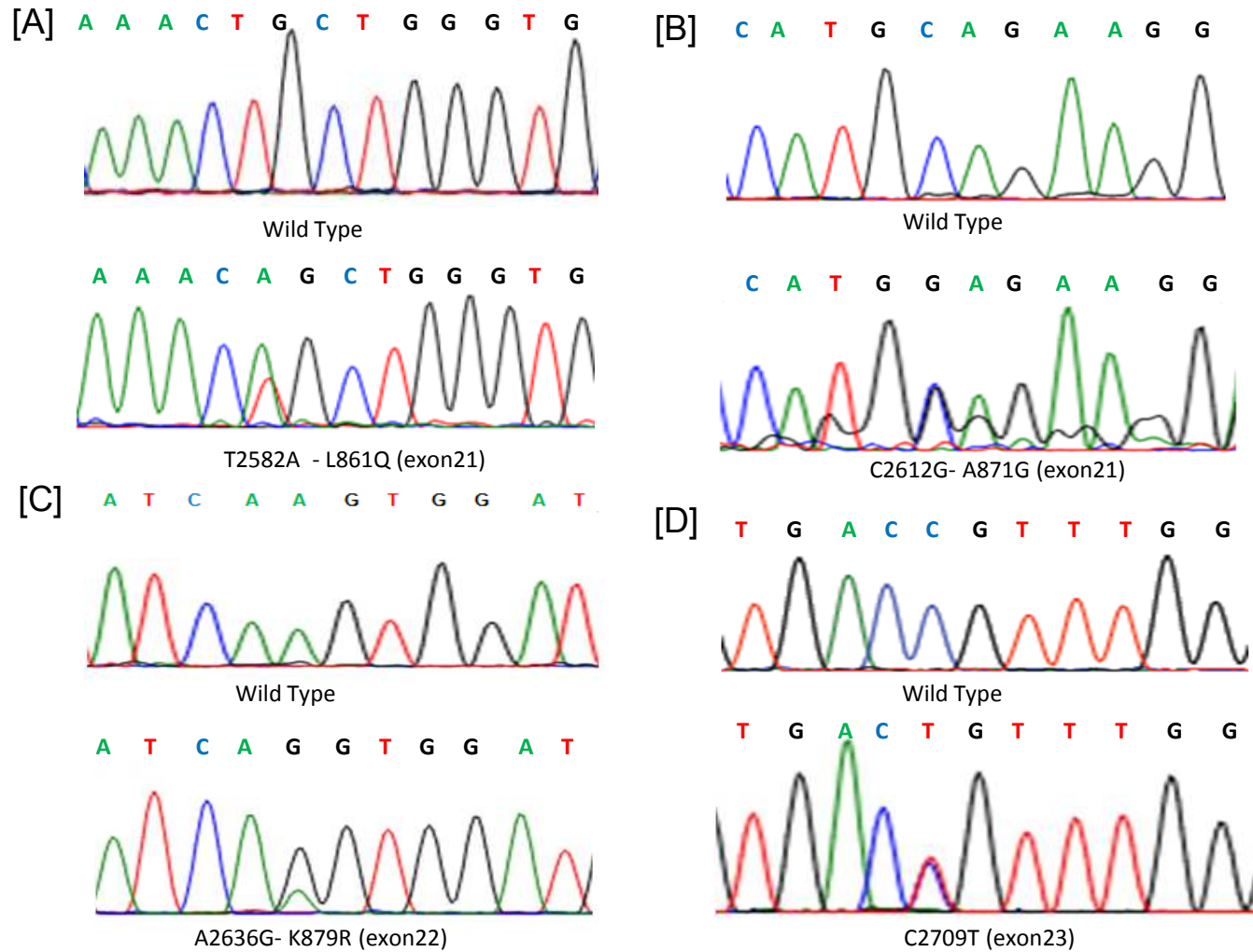
A and B. Base changes indicated as double peaks at positions 2582 (T to A), 2612 (C to G) in exon21. C. Base change at position 2636 (A to G) in exon22 . D. The change at position 2709 (C to T) in exon23 .
