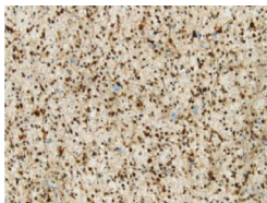
b IDH1 R132H positive
