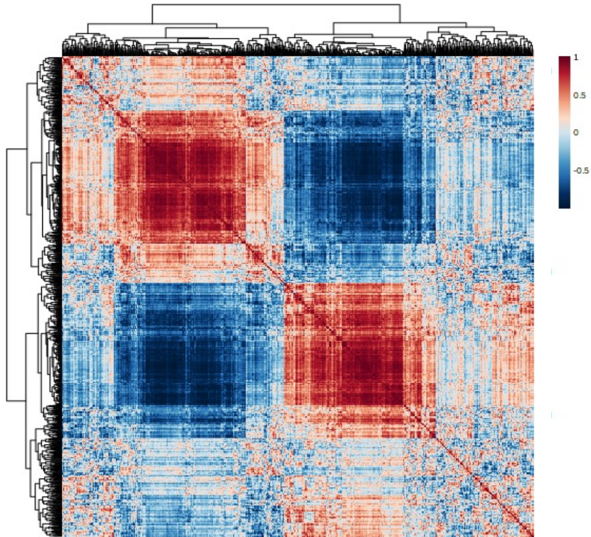
Supplementary figure S7. Correlation heatmap of the LFQ-MS experiment. Pairwise correlations of protein abundances characterizing the relationships between proteins of the global mass spectrometry experiment. Correlations between all proteins, clustering of protein groups and similarly behaving proteins are represented in this protein-protein correlation matrix calculated on the logarithmic intensities. A strong correlation between the technical replicates ( n = 5 ) was observed (red colour) indicating high reproducibility as tested by the Pearson correlation. Negative correlations are represented in a blue color (see legend).
